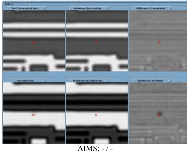
FIGURE 6: Sample of missing defects in DBRt inspection sensitivity settings for >80nm defect size
