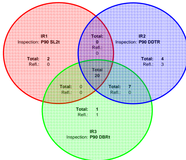
FIGURE 5: Venn diagram for comparison of the 3 different inspection modes with sensitivity settings for >80nm defect size
