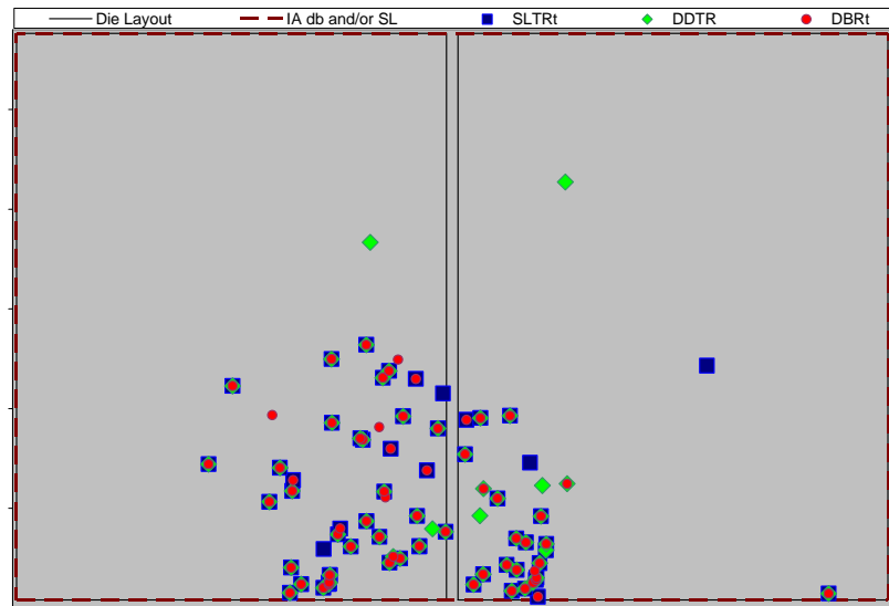
FIGURE 7: Defect Distribution map of all 3 inspections of Mask (B) with sensitivity settings for >60nm defect size
