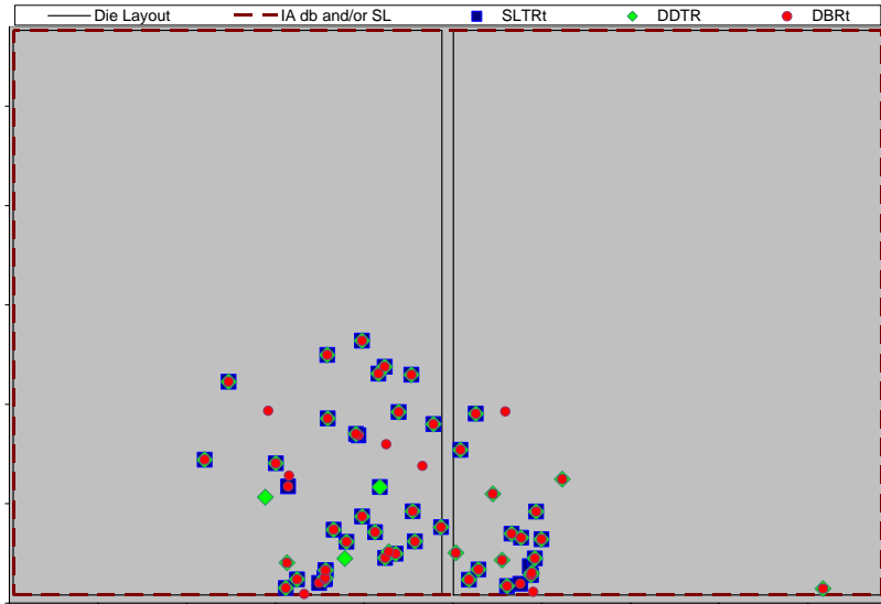
FIGURE 10: Defect Distribution map of all 3 inspections of Mask (B) with sensitivity settings for >80nm defect size
