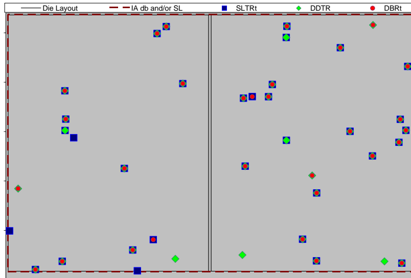
FIGURE 1: Defect Distribution map of all 3 inspections of Mask (A) with sensitivity settings for >60nm defect size
