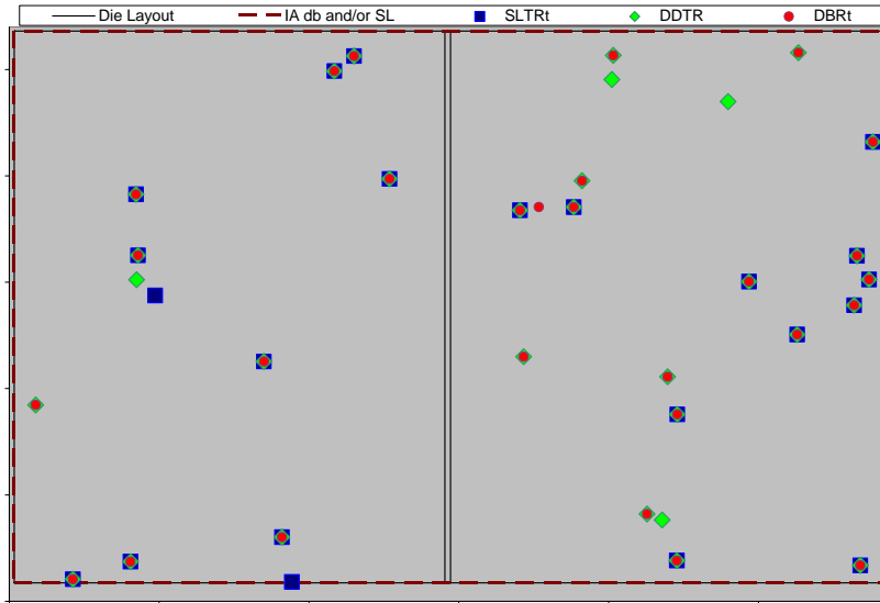
FIGURE 4: Defect Distribution map of all 3 inspections of Mask (A) with sensitivity settings for >80nm defect size
